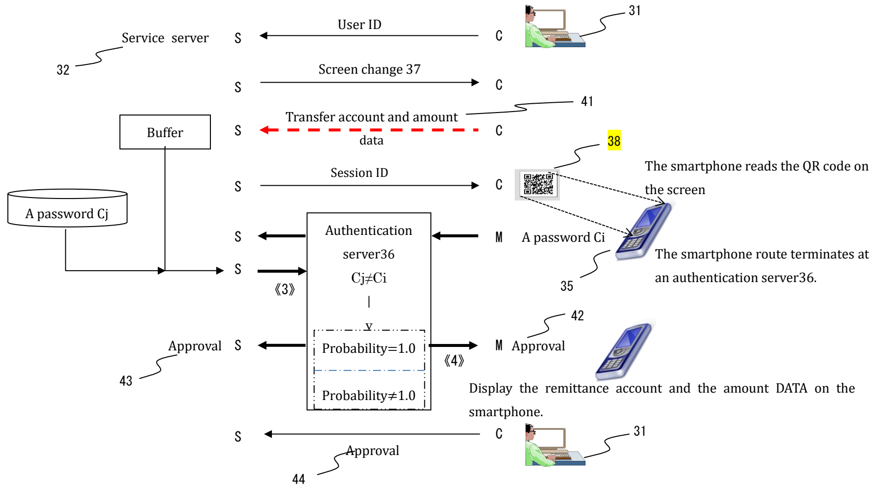
FIG. 4 is a diagram for explaining countermeasures against MITB implemented inside the login mechanism
