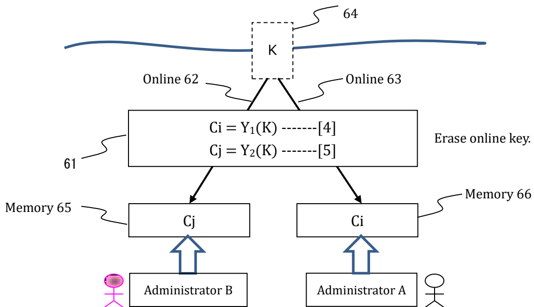
Fig.6: Framework of "Split Knowledge of a key" during operation
